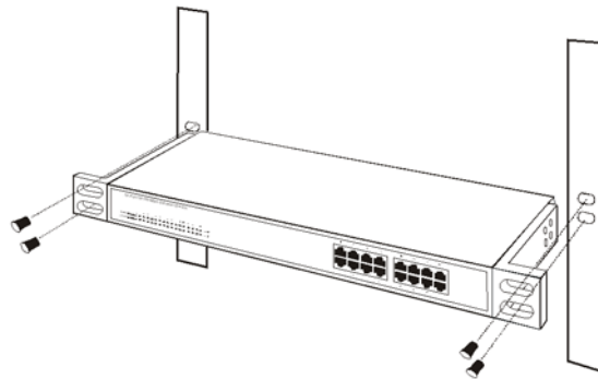
Figure 2. Attach Switch to Rack
